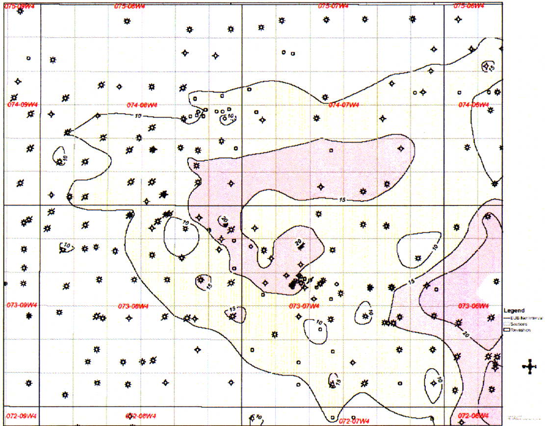
Athabasca Wabiskaw-McMurray Regional geological Study, pg. 104 Wabiskaw B valley-Fill Bitumen Isopach Map
