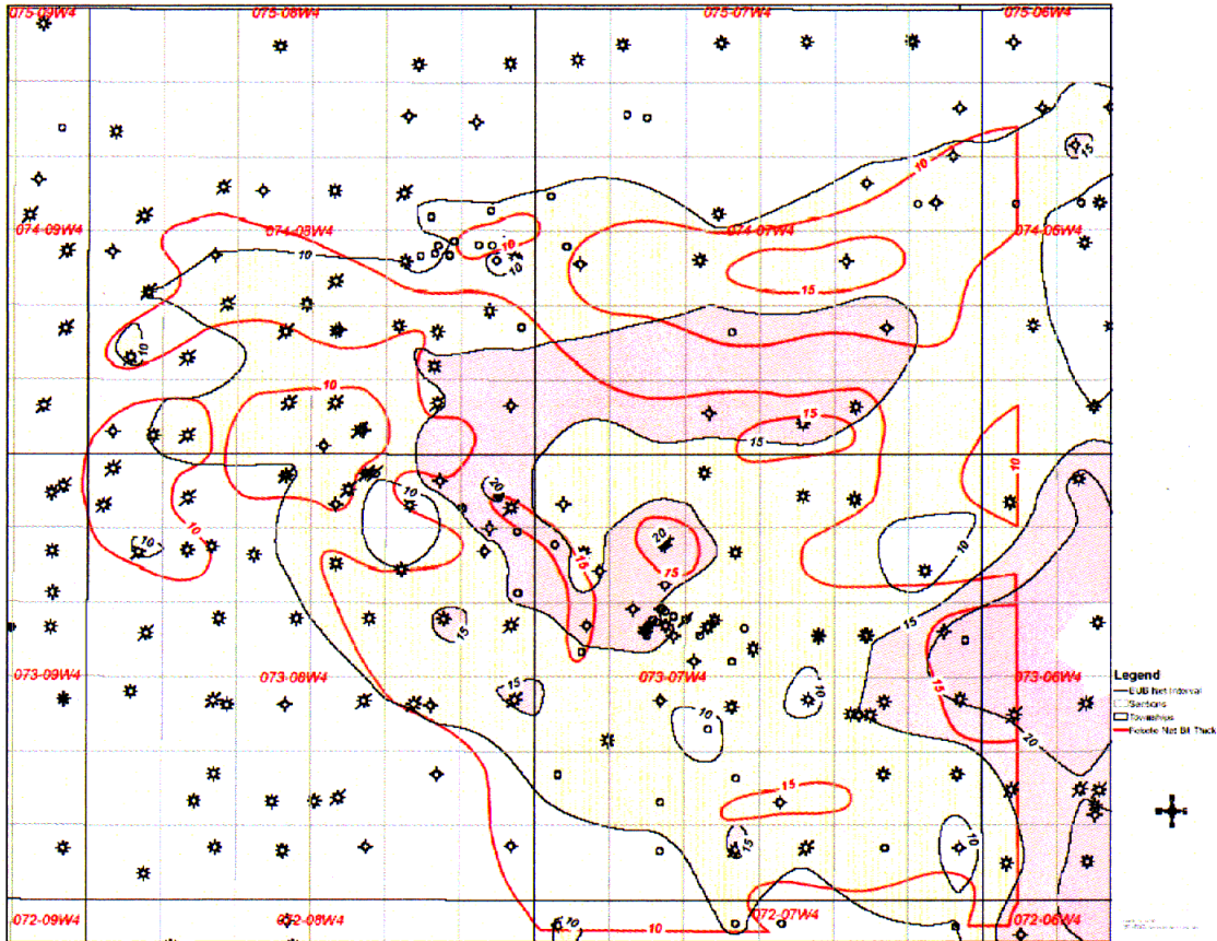
RGS Wabiskaw B Valley fill Bitumen Isopach Map overlain by ISH Net Bitumen Isopach Map
