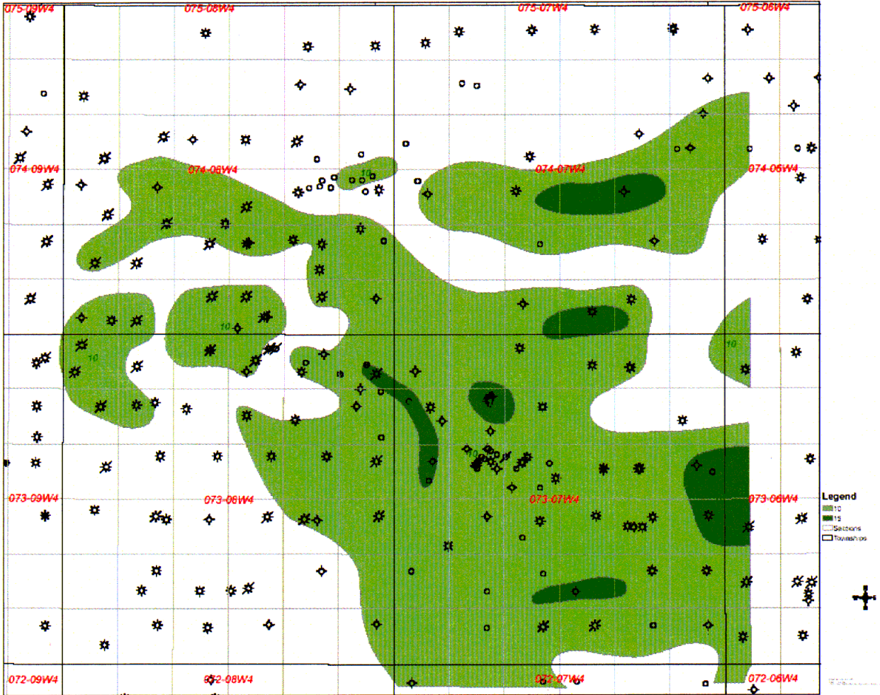
ISH Submission Feb 14, Appendix 2 Figure 9 Wabiskaw B Net Bitumen Isopach Map
