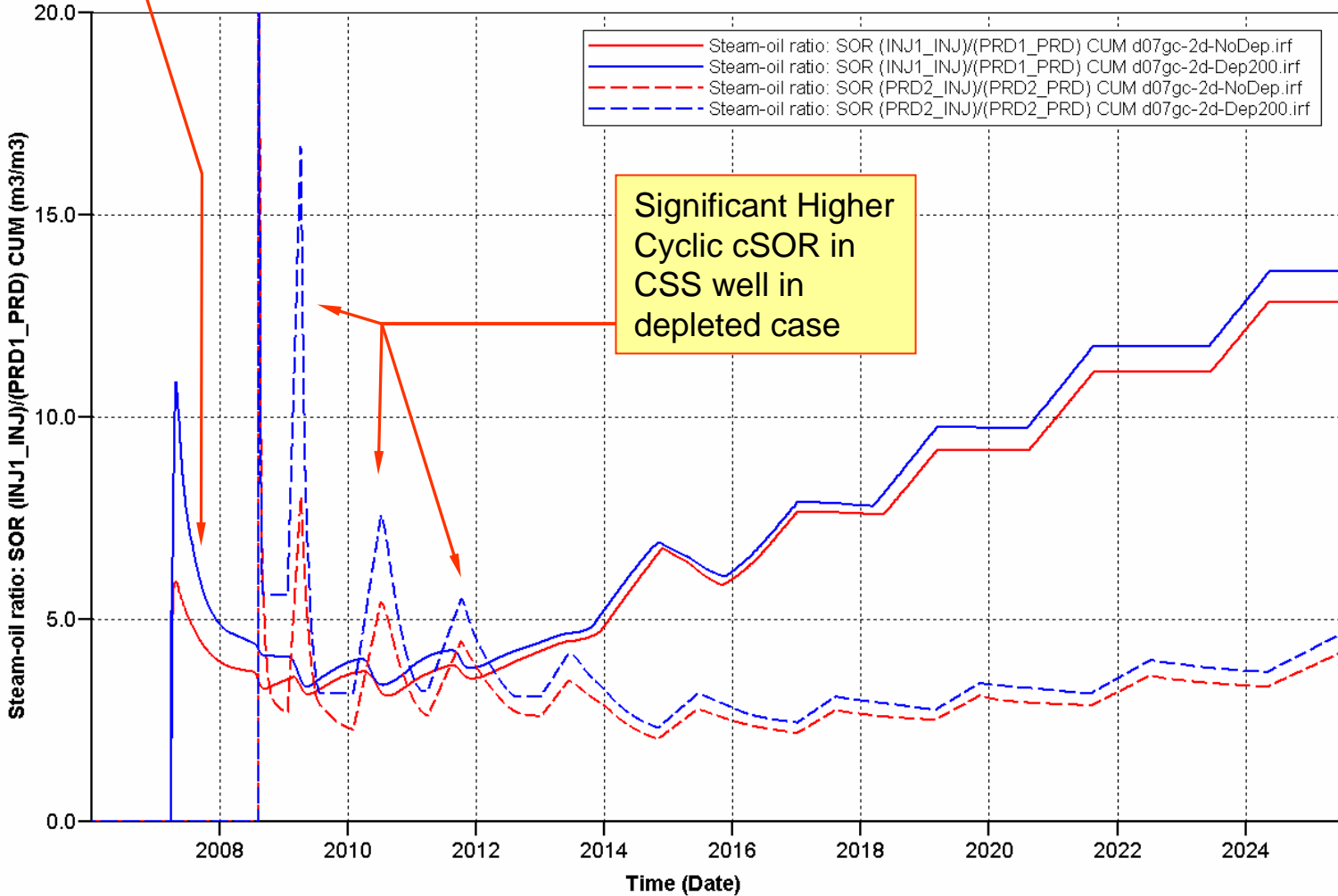
Caribou Hybrid SAGD SOR (INJ1_INJ)/(PRD1_PRD) CUM d07gc-2d-NoDep.irf
